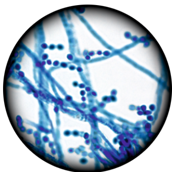
Paecilomyces lilacinus
